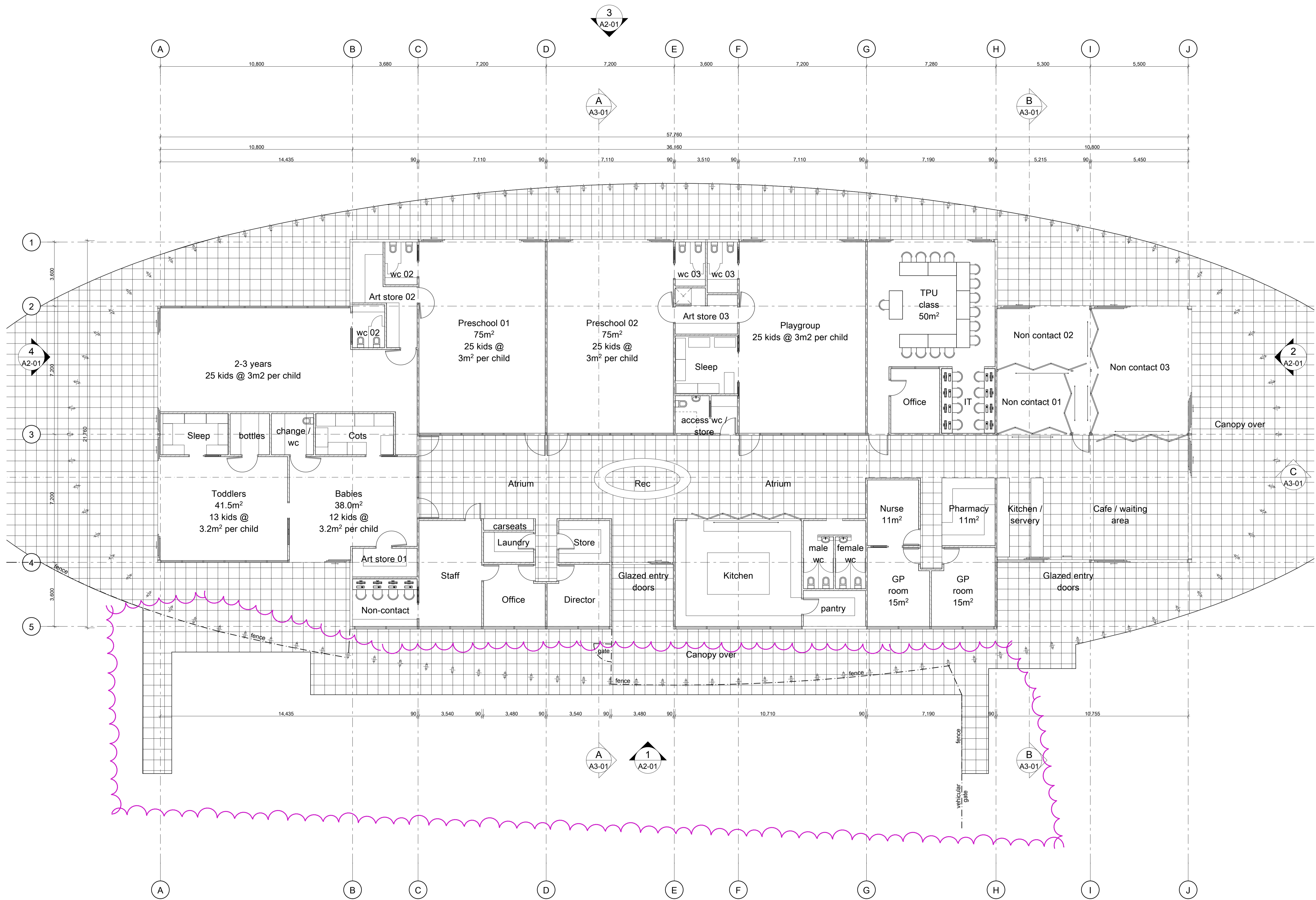
1 Floor Plan 1:100
